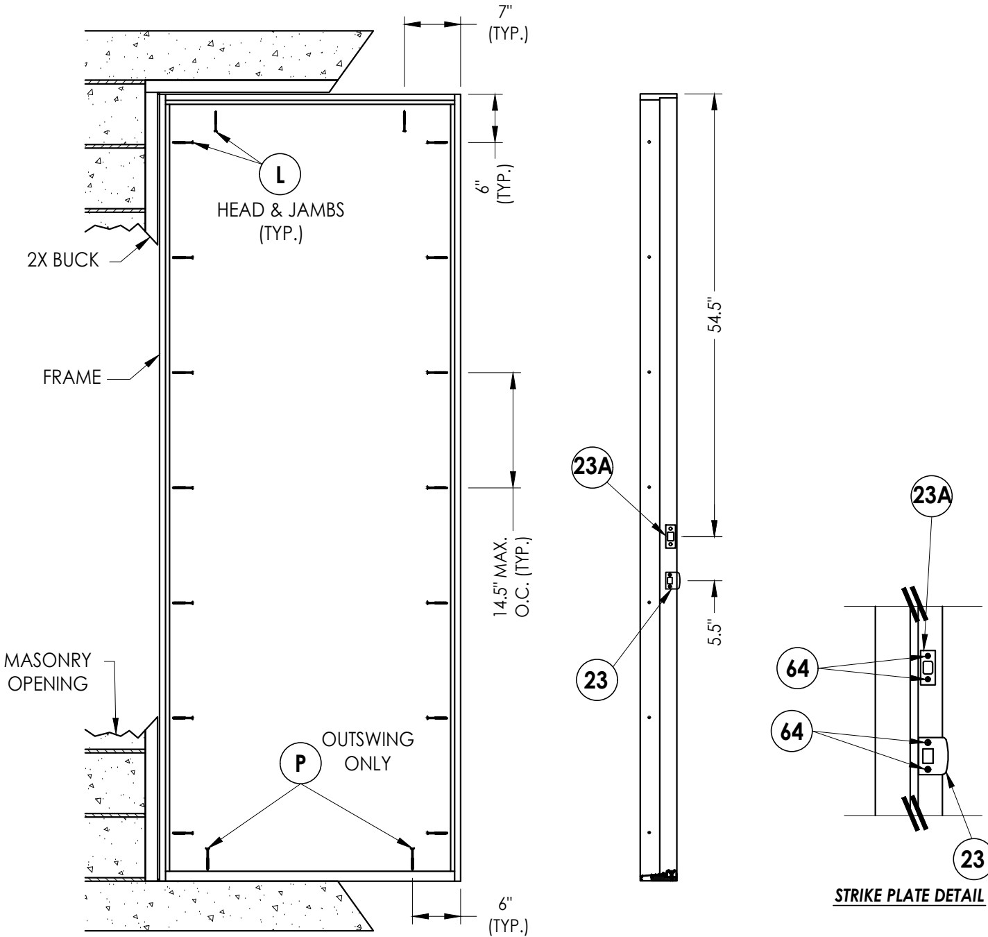
FRAME ANCHORING
