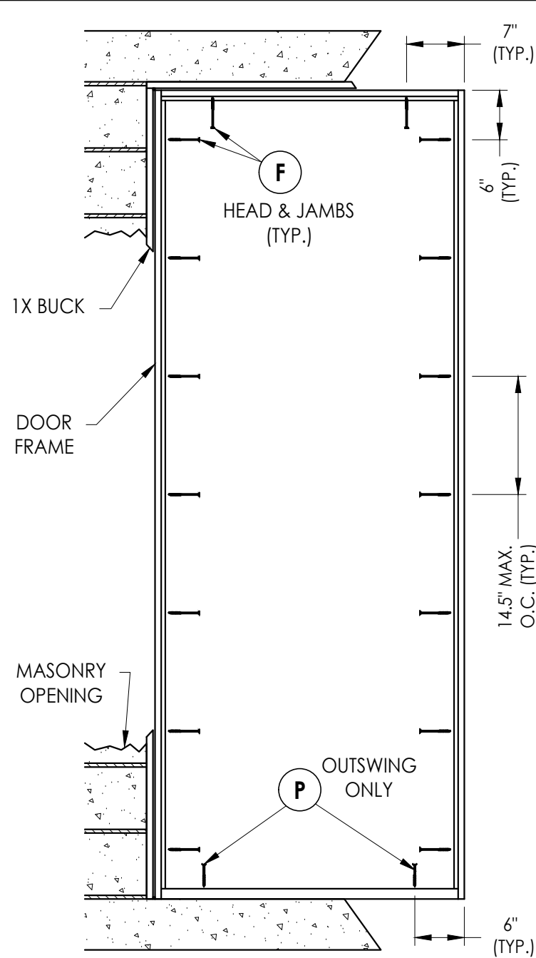
FRAME ANCHORING Masonry 1X buck construction
